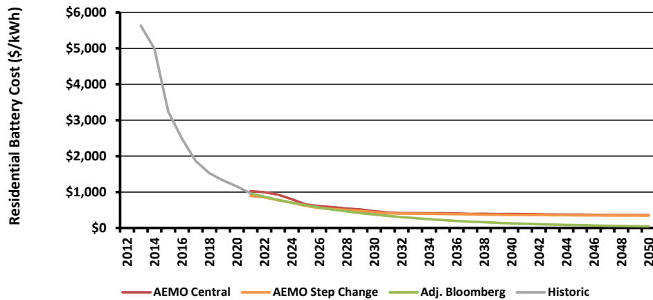
Figure 9 – Residential Battery Storage Cost Outlook by Scenario
